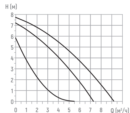
BASIC S 25-8S 180
