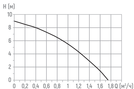
PROMO 15-9A
