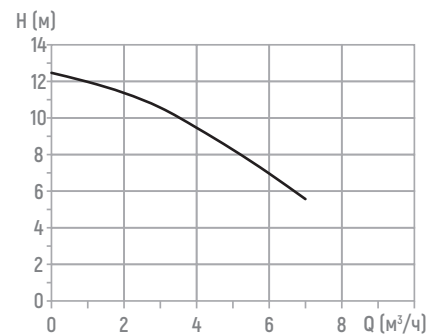
BASIC 25-12 N 180
